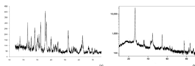
Figure 11. Wide-Angle X-Ray Diffraction (WAXD) analysis of malignant human cancer cells and tissues (a) before and (b) after irradiating of synchrotron radiation in transformation process to benign human cancer cells and tissues with the passing of time [1-170]
