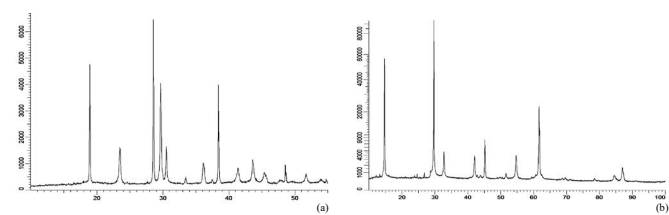
Figure 9. X-Ray Diffraction (XRD) analysis of malignant human cancer cells and tissues (a) before and (b) after irradiating of synchrotron radiation in transformation process to benign human cancer cells and tissues with the passing of time [1-170]
