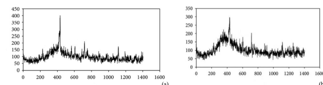
Figure 4. Wide-Angle X-Ray Scattering (WAXS) analysis of malignant human cancer cells and tissues (a) before and (b) after irradiating of synchrotron radiation in transformation process to benign human cancer cells and tissues with the passing of time [1-170]
