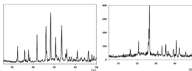
Figure 3. Fluctuation X-Ray Scattering (FXS) analysis of malignant human cancer cells and tissues (a) before and (b) after irradiating of synchrotron radiation in transformation process to benign human cancer cells and tissues with the passing of time [1-170]
