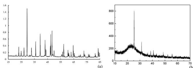
Figure 5. Grazing-Incidence Small-Angle X-Ray Scattering (GISAXS) analysis of malignant human cancer cells and tissues (a) before and (b) after irradiating of synchrotron radiation in transformation process to benign human cancer cells and tissues with the passing of time [1-170]
