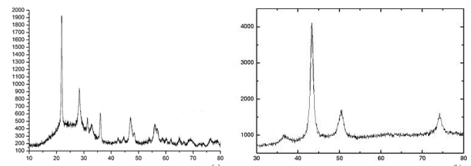
Figure 10. Powder X-Ray Diffraction (PXRD) analysis of malignant human cancer cells and tissues (a) before and (b) after irradiating of synchrotron radiation in transformation process to benign human cancer cells and tissues with the passing of time [1-170]
