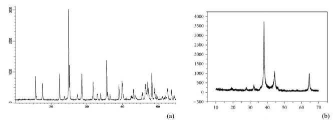
Figure 8. Grazing-Incidence Small-Angle Neutron Scattering (GISANS) analysis of malignant human cancer cells and tissues (a) before and (b) after irradiating of synchrotron radiation in transformation process to benign human cancer cells and tissues with the passing of time [1-170]
