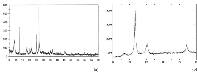
Figure 2. Ultra-Small Angle X-Ray Scattering (USAXS) analysis of malignant human cancer cells and tissues (a) before and (b) after irradiating of synchrotron radiation in transformation process to benign human cancer cells and tissues with the passing of time [1-170]
