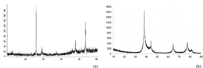
Figure 6. Grazing-Incidence Wide-Angle X-Ray Scattering (GIWAXS) analysis of malignant human cancer cells and tissues (a) before and (b) after irradiating of synchrotron radiation in transformation process to benign human cancer cells and tissues with the passing of time [1-170]
