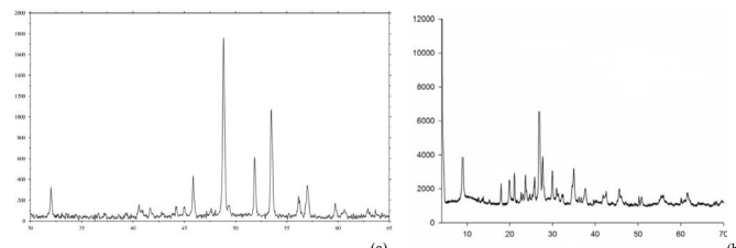
Figure 13. Energy-Dispersive X-Ray Diffraction (EDXRD) analysis of malignant human cancer cells and tissues (a) before and (b) after irradiating of synchrotron radiation in transformation process to benign human cancer cells and tissues with the passing of time [1-170]
