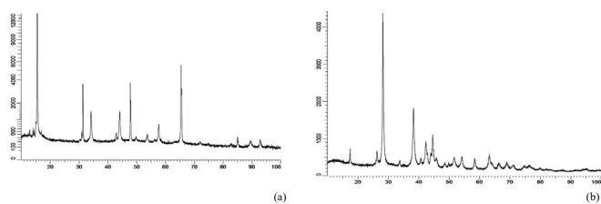
Figure 1. Small-Angle X-Ray Scattering (SAXS) analysis of malignant human cancer cells and tissues (a) before and (b) after irradiating of synchrotron radiation in transformation process to benign human cancer cells and tissues with the passing of time [1-170]
