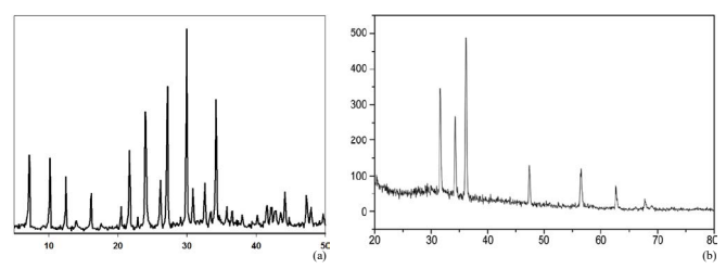
Figure 7. Small-Angle Neutron Scattering (SANS) analysis of malignant human cancer cells and tissues (a) before and (b) after irradiating of synchrotron radiation in transformation process to benign human cancer cells and tissues with the passing of time [1-170]
