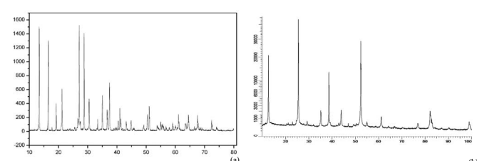
Figure 12. Grazing-Incidence X-Ray Diffraction (GIXD) analysis of malignant human cancer cells and tissues (a) before and (b) after irradiating of synchrotron radiation in transformation process to benign human cancer cells and tissues with the passing of time [1-170]
